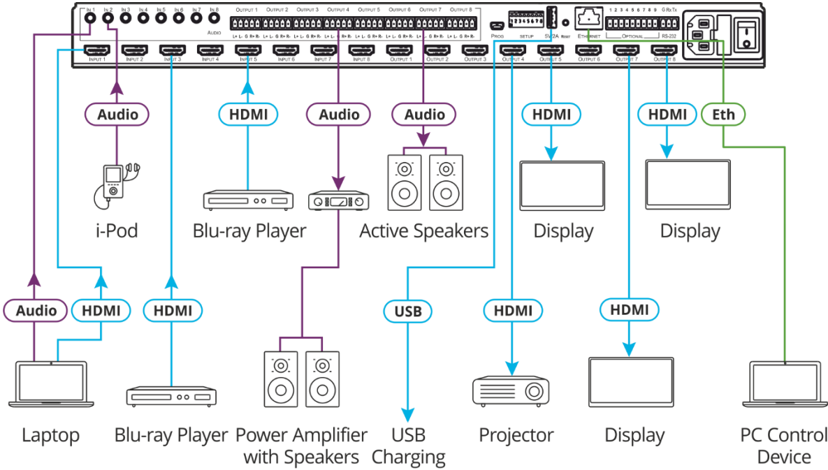
Figure 3: Connecting to the VS-88UHDA Rear Panel
