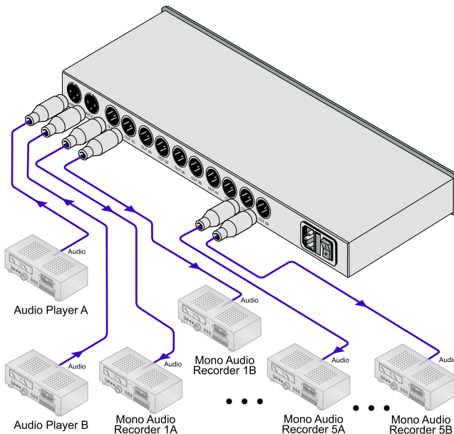
Figure 3: Connecting the VM-1110xl as a 2x1:5 Mono DA
