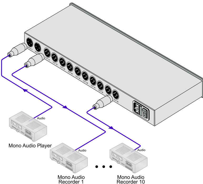
Figure 2: Connecting the VM-1110xl as a 1:10 Mono DA
