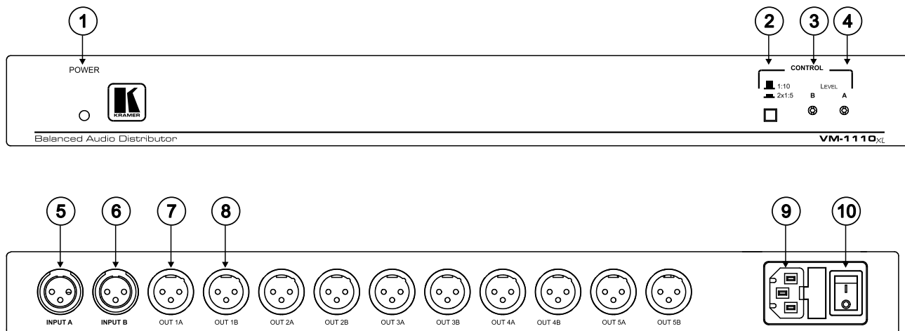
Figure 1: VM-1110xl Balanced Audio Distributor
