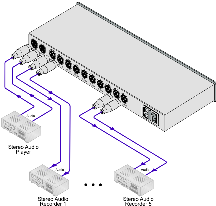
Figure 4: Connecting the VM-1110xl as a 1:5 Stereo DA
