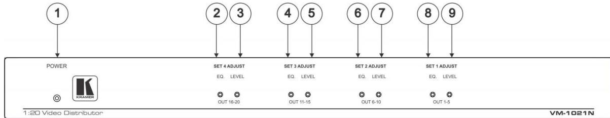
Figure 1: VM-1021N 1:20 Video Distributor Front Panel
