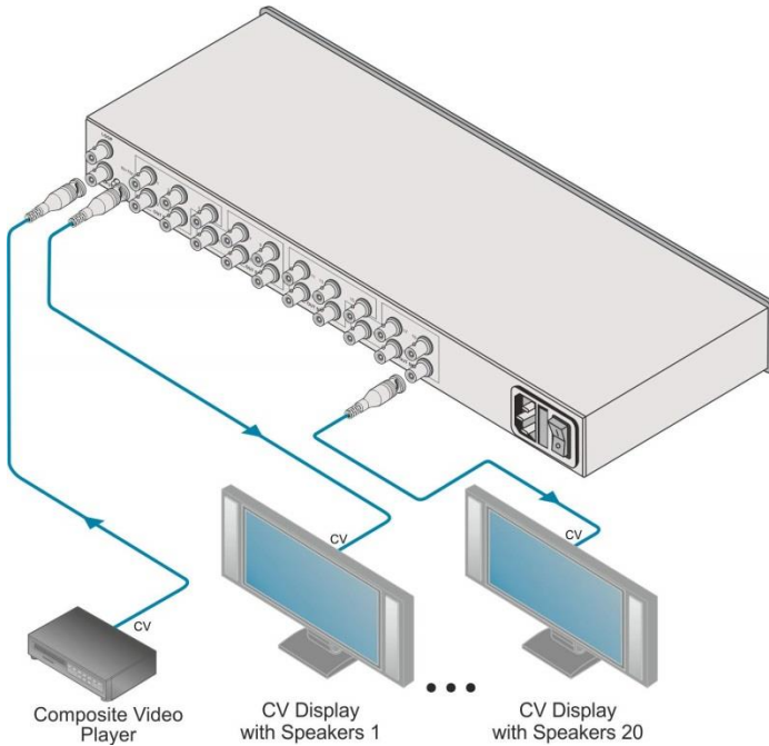
Figure 3: Connecting the VM-1021N
