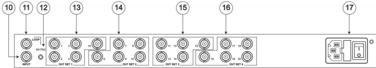
Figure 2: VM-1021N 1:20 Video Distributor Rear Panel
