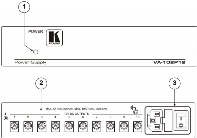
Figure 2: VA-102P12 10-Output 12V DC Power Supply
