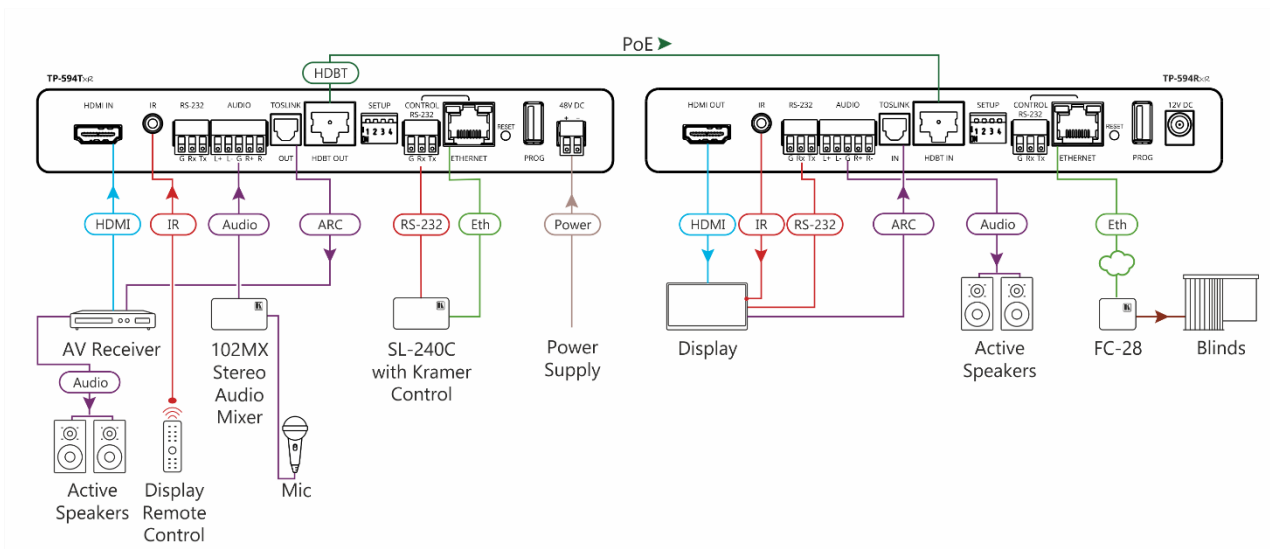
Figure 3: Connecting to the TP-594Txr Rear Panel
