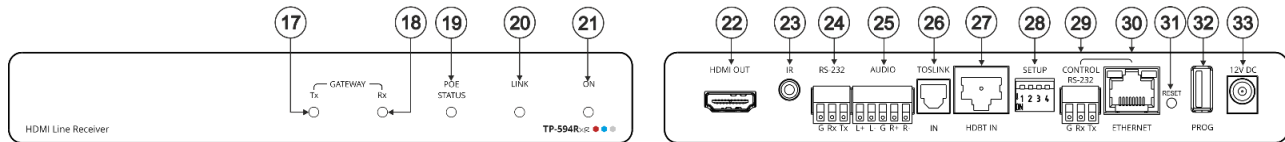
Figure 2: TP-594Rxx HDMI Line Receiver
