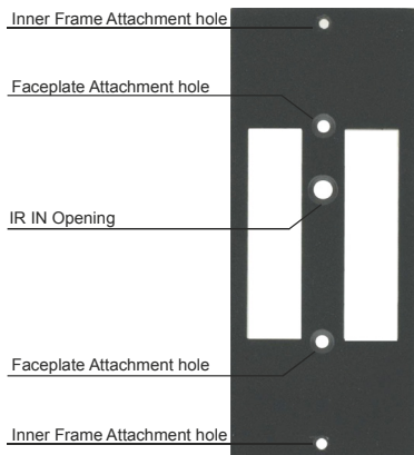
Figure 4: T-RC8IR (P/N: 80-000599)
