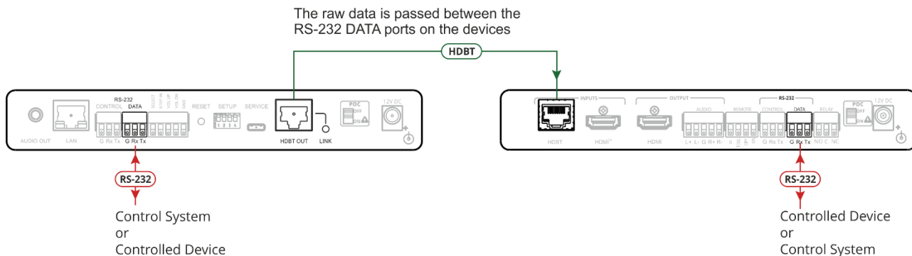
Figure 9: Controlling a Sink Device on the Receiver via the Data Ports
