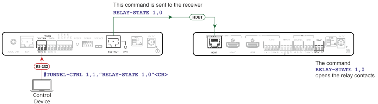
Figure 7: Controlling the Receiver via a Control System
