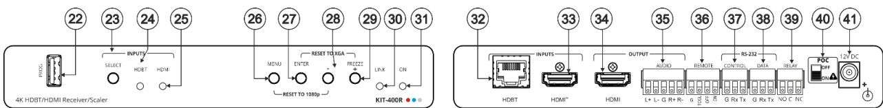
Figure 2: KIT-400R 4K HDBT/HDMI Receiver/Scaler
