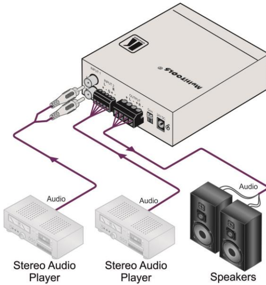
Figure 2: Connecting the 907xl Power Amplifier/Mixer
