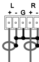
Figure 4: Connecting an Unbalanced Input to the Balanced Stereo Audio Input
