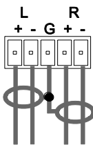
Figure 3: Connecting a Balanced Input to the Balanced Stereo Audio Input
