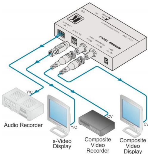
Figure 2: Connecting the 810 Color Bar/Audio Generator
