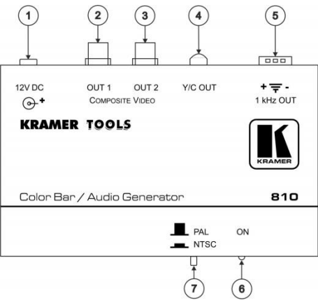
Figure 1: 810 Color Bar/Audio Generator
