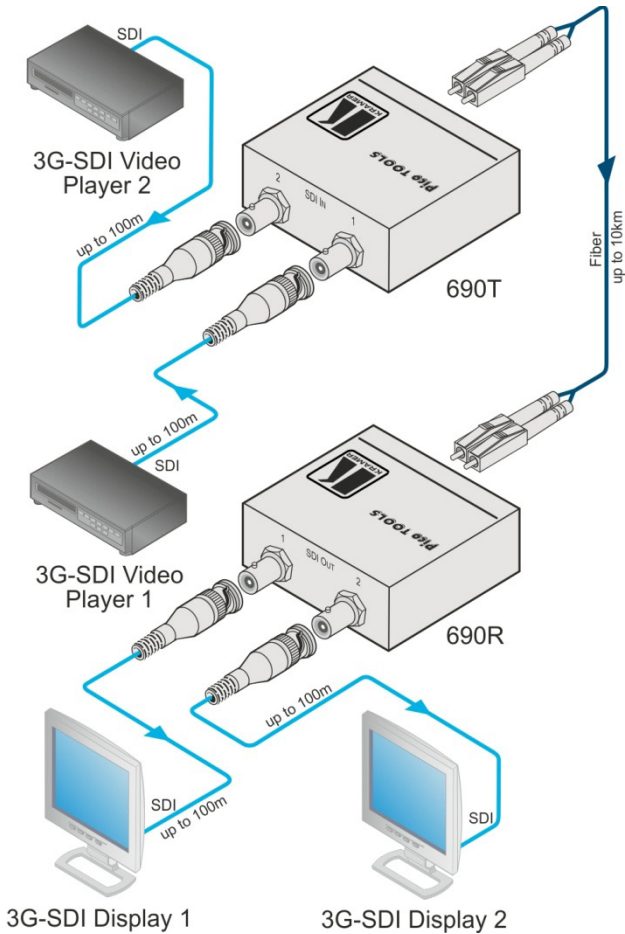
Figure 3: Connecting the 690T and/or 690R
