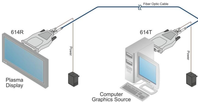
Figure 2: Connecting the 614T/614R
