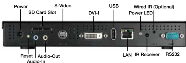
SignShow D5000 Inputs and outputs
