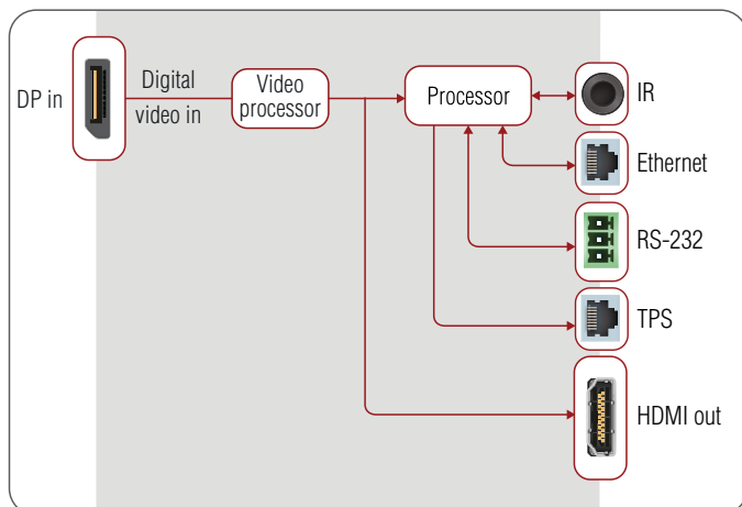
Port diagram
