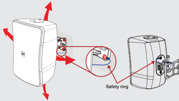
Knuckle Bracket
