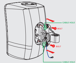
Back Cover
