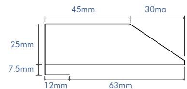
Smart-View frame cross section
