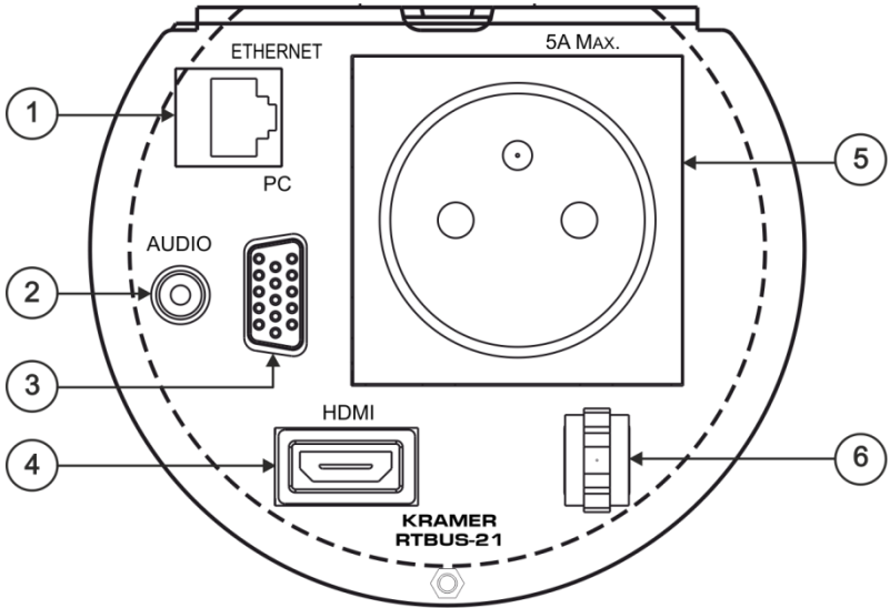
Figure 2: RTBUS-21 Connecting Surface
