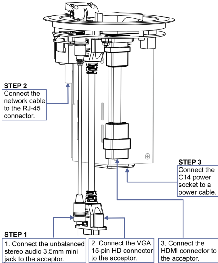
Figure 3: Connecting the Cables
