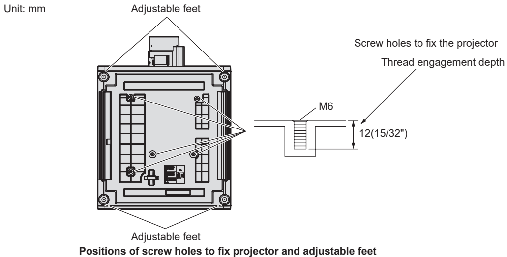
Positions of screw holes to fix projector and adjustable feet
